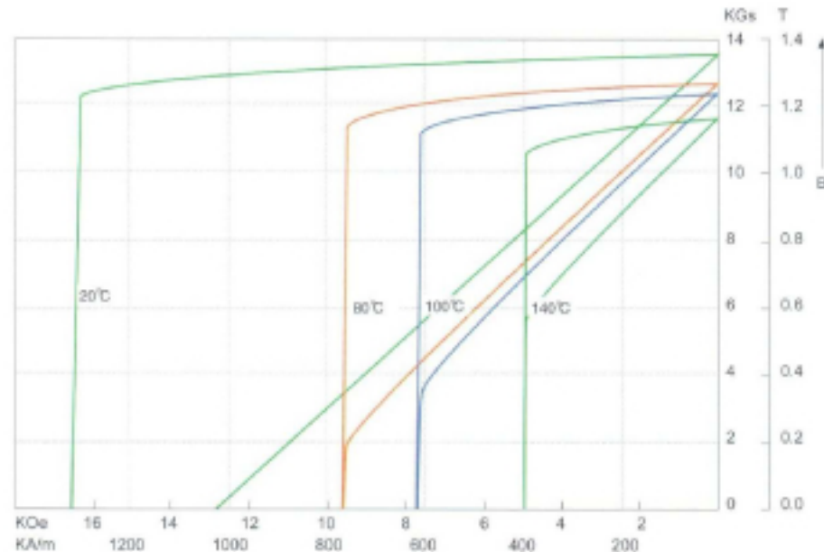
No Dy 44HF Variable temperature curve
